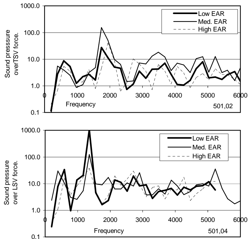
Figure 6. The radiated sound pressure divided by the TSV force (above) and by the LSV force (below). Data points (at 196Hz intervals) are omitted for clarity.
