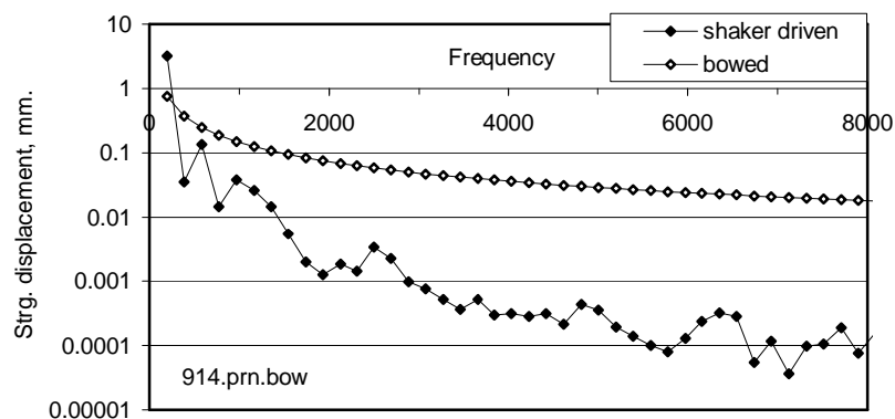
Figure 1. String displacement of a shaker driven open G string compared to that of the bowed string. The peak heights at the harmonics are shown as points (at 196Hz intervals), and the points are joined by lines to improve the clarity of presentation.
