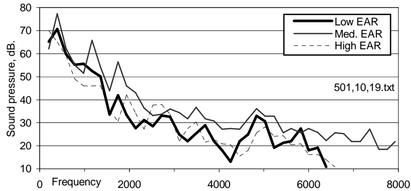
Figure 5. Sound pressure level radiated (uncalibrated), equal first harmonic string displacement. Shaker driven G string. Shown for violins of differing EAR. Data points (at 196Hz intervals) omitted for clarity
