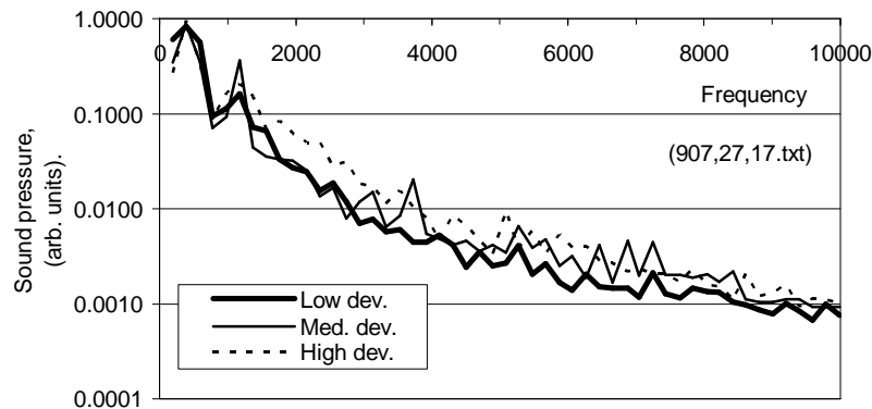
Figure 7. Sound pressure radiated (uncalibrated), equal first harmonic string displacement. Shaker driven G string. Shown for violins of differing deviation. Data points (at 196Hz intervals) omitted for clarity.
